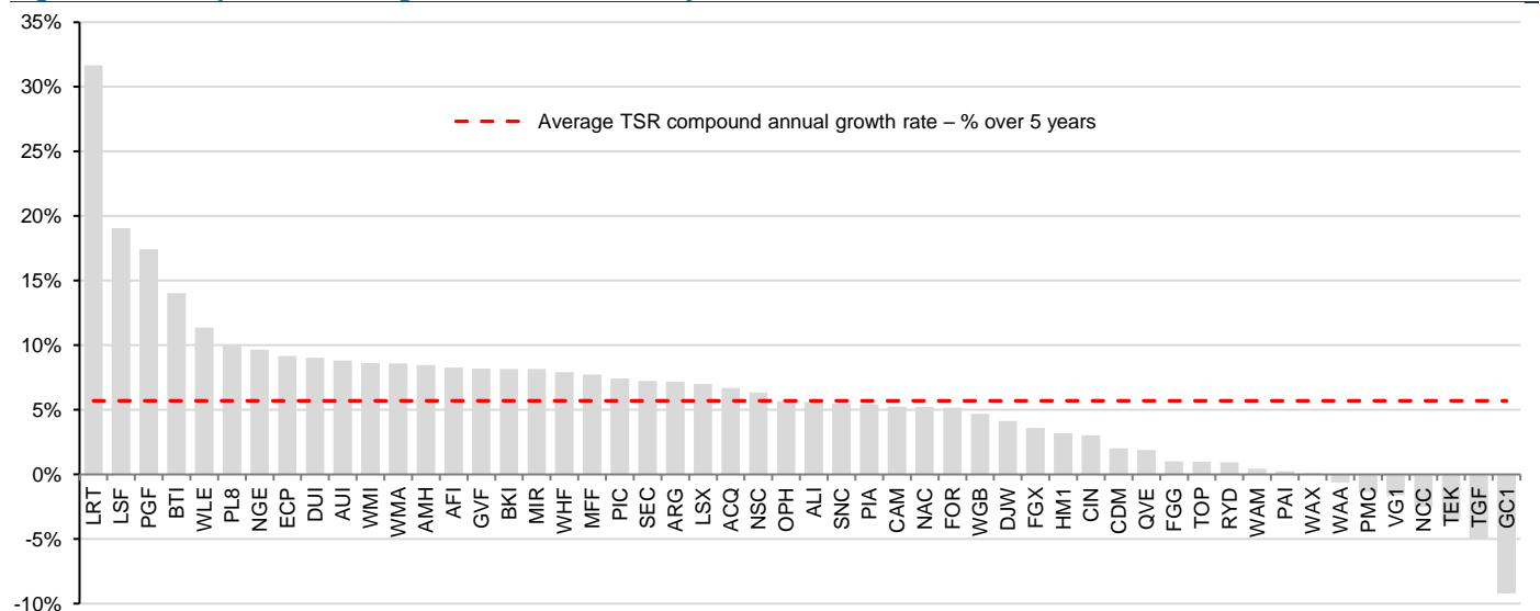
Fig.28: TSR compound annual growth rate – % over 5 years
