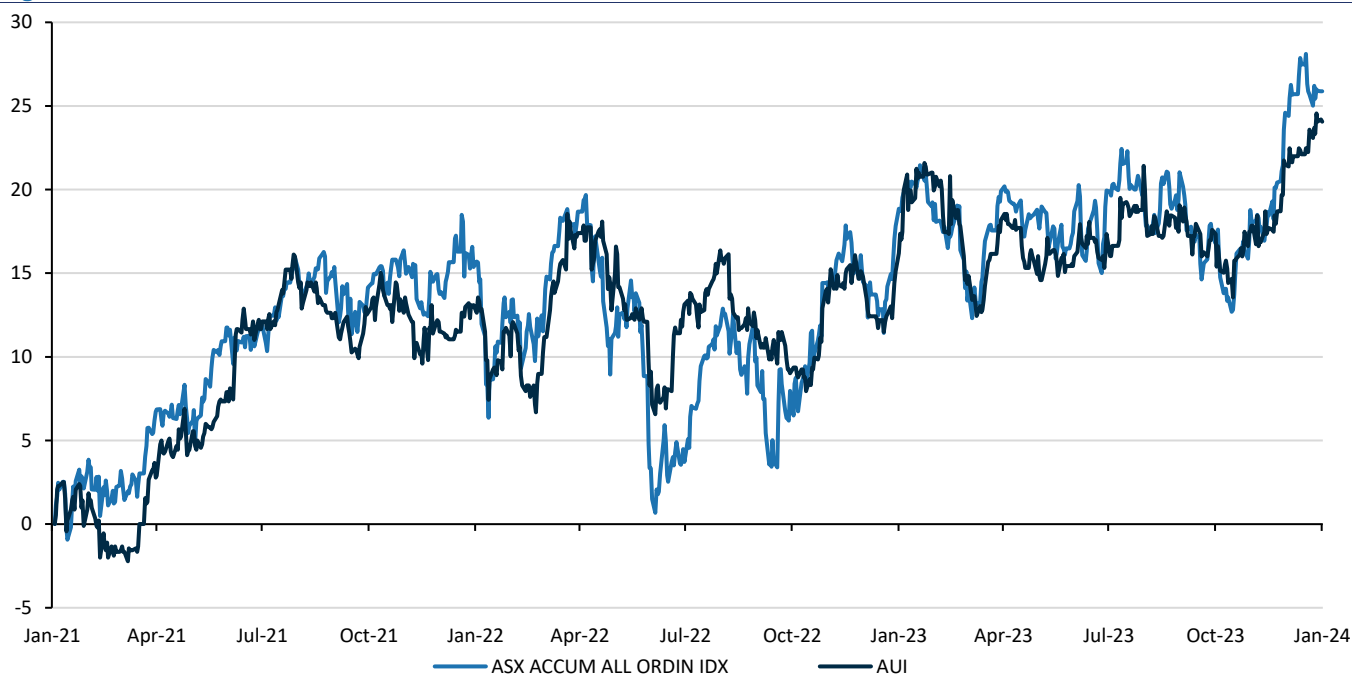
Fig.5: AUI TSR vs All Ords Accum. Index
